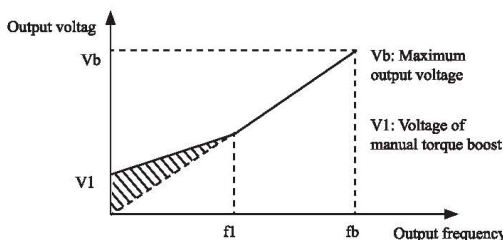
Figure 4-5 Manual torque boost
